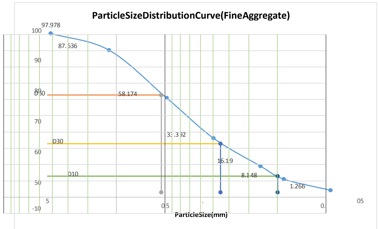
Figure 1: Particle Distribution Curve Results on Sieve Analysis (Fine Aggregate)
