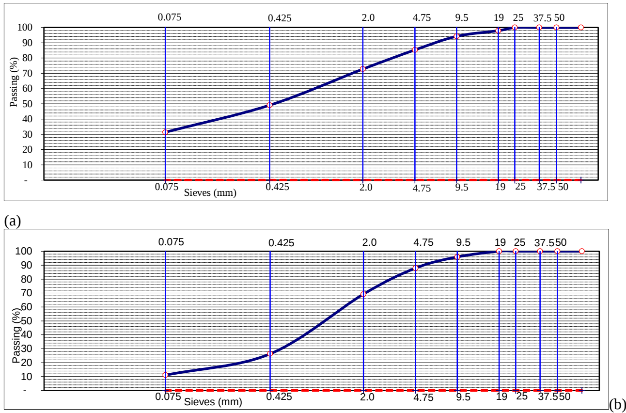
Figure 2: (a) Graph of percentage passing (%) against sieve sizes (mm) for sample location 1A (b) Graph of percentage passing (%) against sieve sizes (mm) for sample location 1B
